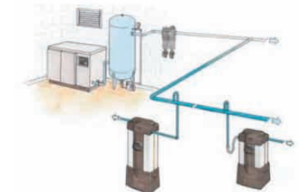
A Regenerative Desiccant Dryer System Installed to Supply Control Air for a CNC Machining Center.
